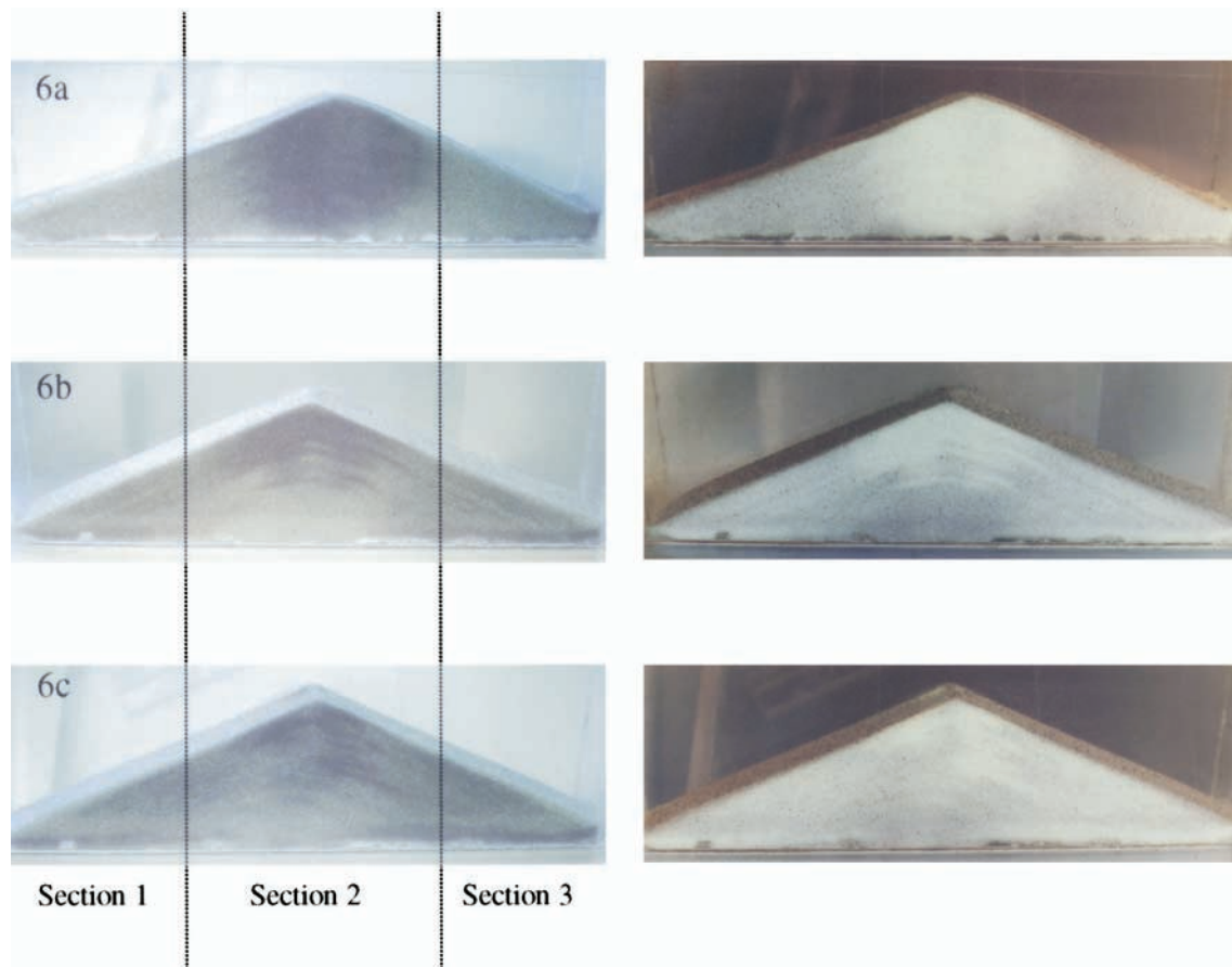
Fig. 6. Poured binary mixtures of glass spheres, 47% small ( 300\ \mu\text{m} ) and 53% large ( 800\ \mu\text{m} ). The small grains appear black in the photos on the left side and light green in the negative images on the right side used to highlight the distribution of beads. The three photos represent piles poured at differing velocities (a) 50\ \text{g s}^{-1} , (b) 3.7\ \text{g s}^{-1} , and (c) 0.83\ \text{g s}^{-1} . The dashed lines show the approximate positions of where the piles were sectioned for the data presented in Fig. 7.
