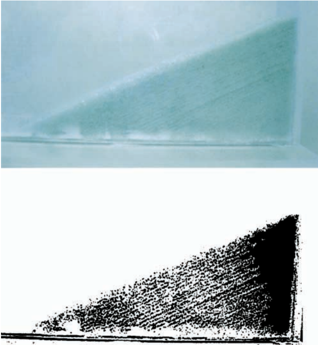
Fig. 4. Upper, photograph of a binary mixture of a 50:50 mixture of 300- and 800- \mu\text{m} glass spheres. Banding caused by segregation can be seen parallel to the slope angle. The lower diagram is a textured image used to highlight the dark areas and better show the banding.
