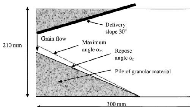
Fig. 2. Schematic diagram of the Hele-Shaw cell used in the experiments; the maximum angle of stability and angle of repose are illustrated.
