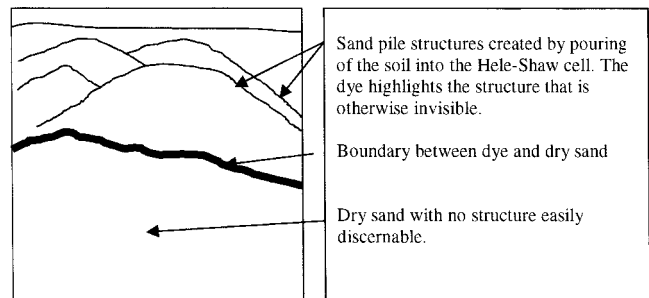
Fig. 3. An overlay of the structures caused by packing that can be observed in a photograph of a repacked sandy soil presented in Fig. 1d of Wang et al. (2002).
