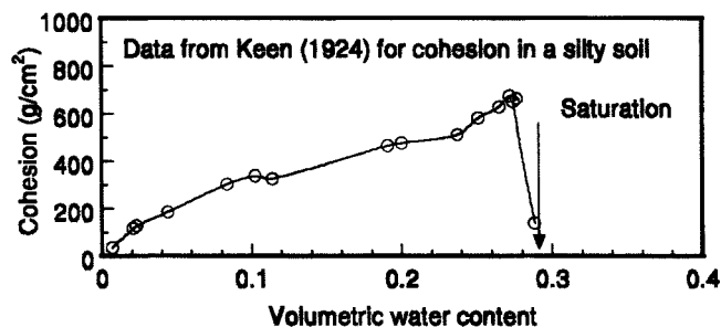
Fig. 8. Cohesion data for a silty soil as a function of water content. Our suggestion is that the best uniform mixing is achieved below saturation but above air dry, where the cohesion aids the mixing.
