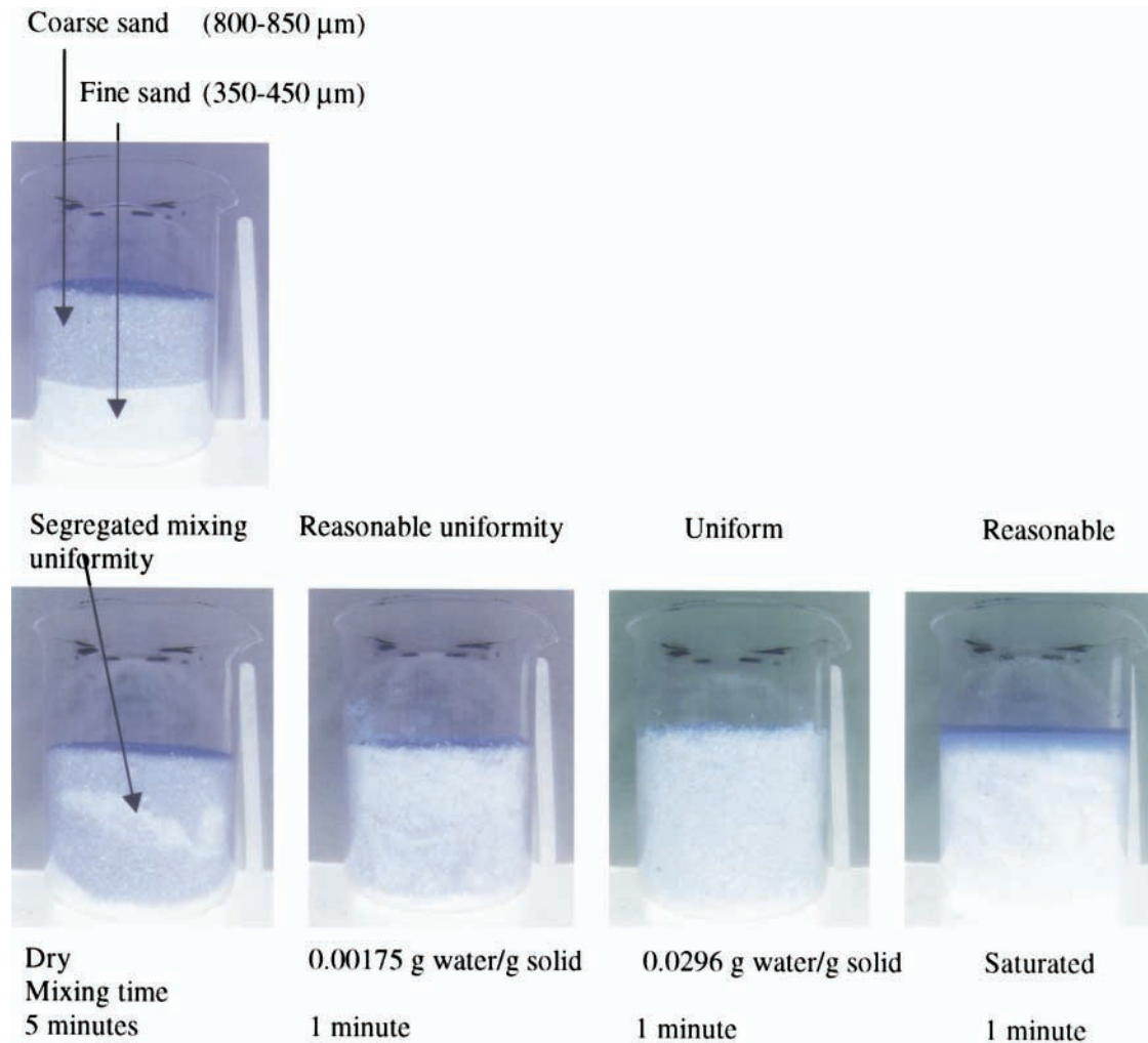
Fig. 9. Pictures of two sands of different colors. We used negative imagery to highlight the contrast between the color of the grains. Shown are the initial dry and segregated state, air dry mixed, and results of mixing with increasing water contents. Thorough mixing occurs at a gravimetric water content of about 0.03. At saturation the mixing is better than air dry, but percolation of the small particles begins to occur.
