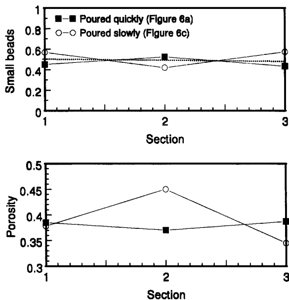
Fig. 7. Upper, the mass fraction of small beads relative to large in Sections 1, 2, and 3, corresponding to Fig. 6a and 6c. The lower diagram shows the respective porosity values.
