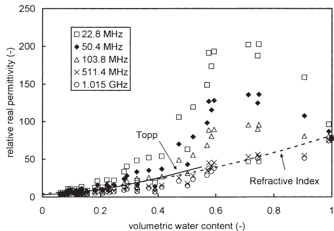
Fig. 2. Real permittivity as a function of water content for bentonite. Results are from the network analyzer for five different frequencies. The \epsilon_r(\theta) relationships according to Topp and the refractive index model are also shown.
