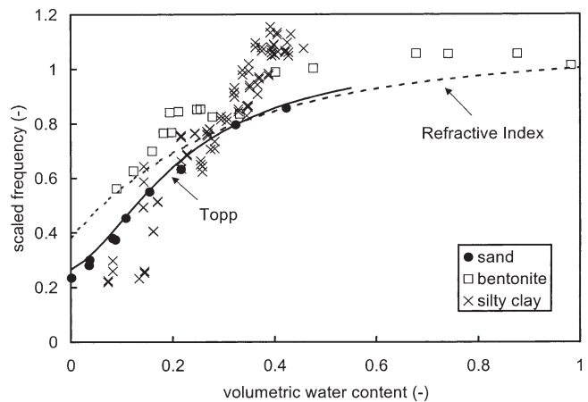
Fig. 6. Scaled frequency as a function of water content. Results for fine quartz sand, bentonite, and a saline silty clay soil. The curves were calculated by combining the respective \epsilon_a(\theta) relationships with the electric circuit model that assumes no dielectric losses (Eq. [8]).
